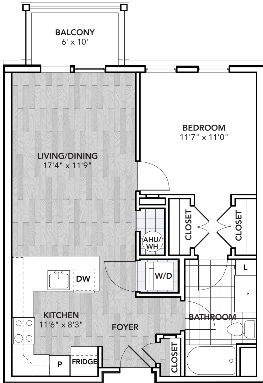
MODEL A1.2 • 716 SQ FT ONE BEDROOM • ONE BATH
