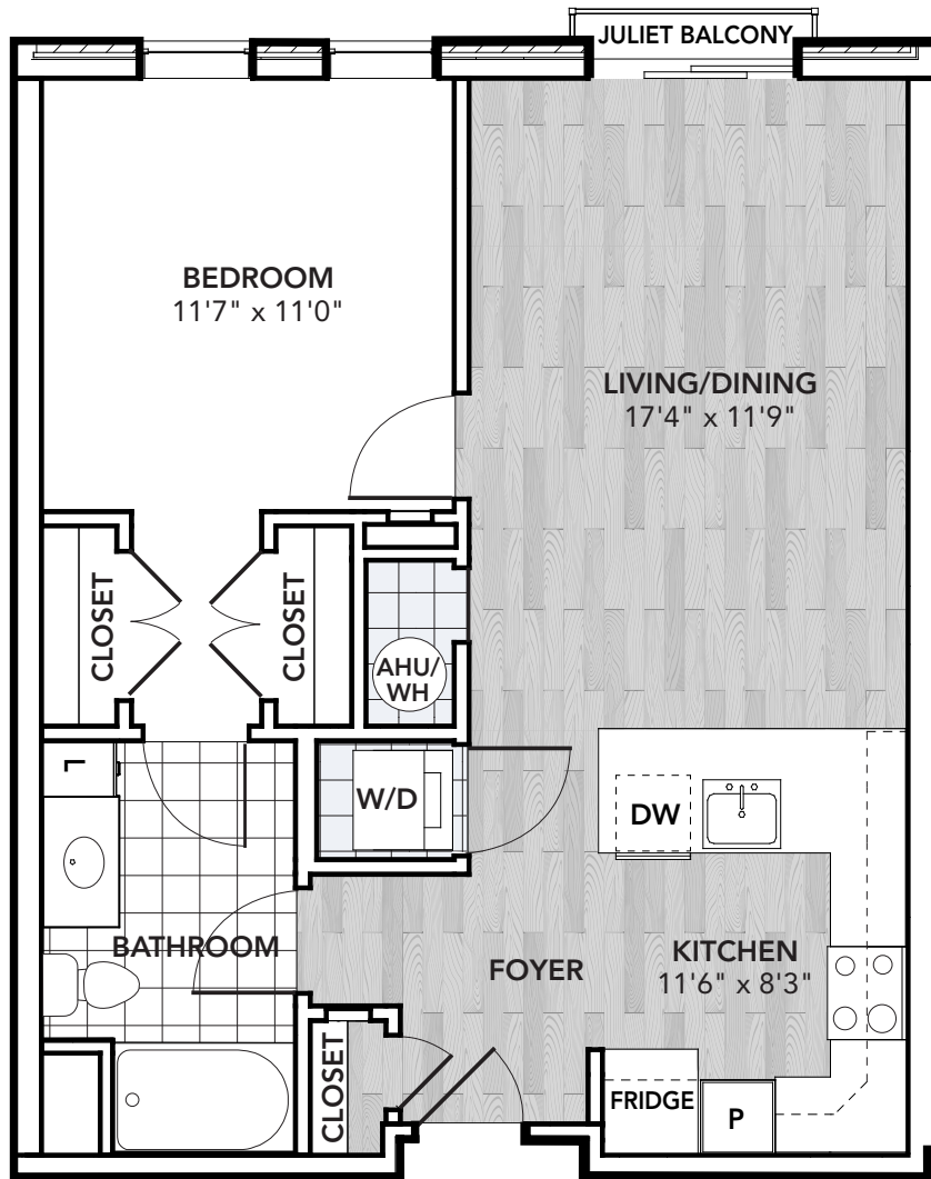
MODEL A1.1 • 726 SQ FT ONE BEDROOM • ONE BATH
