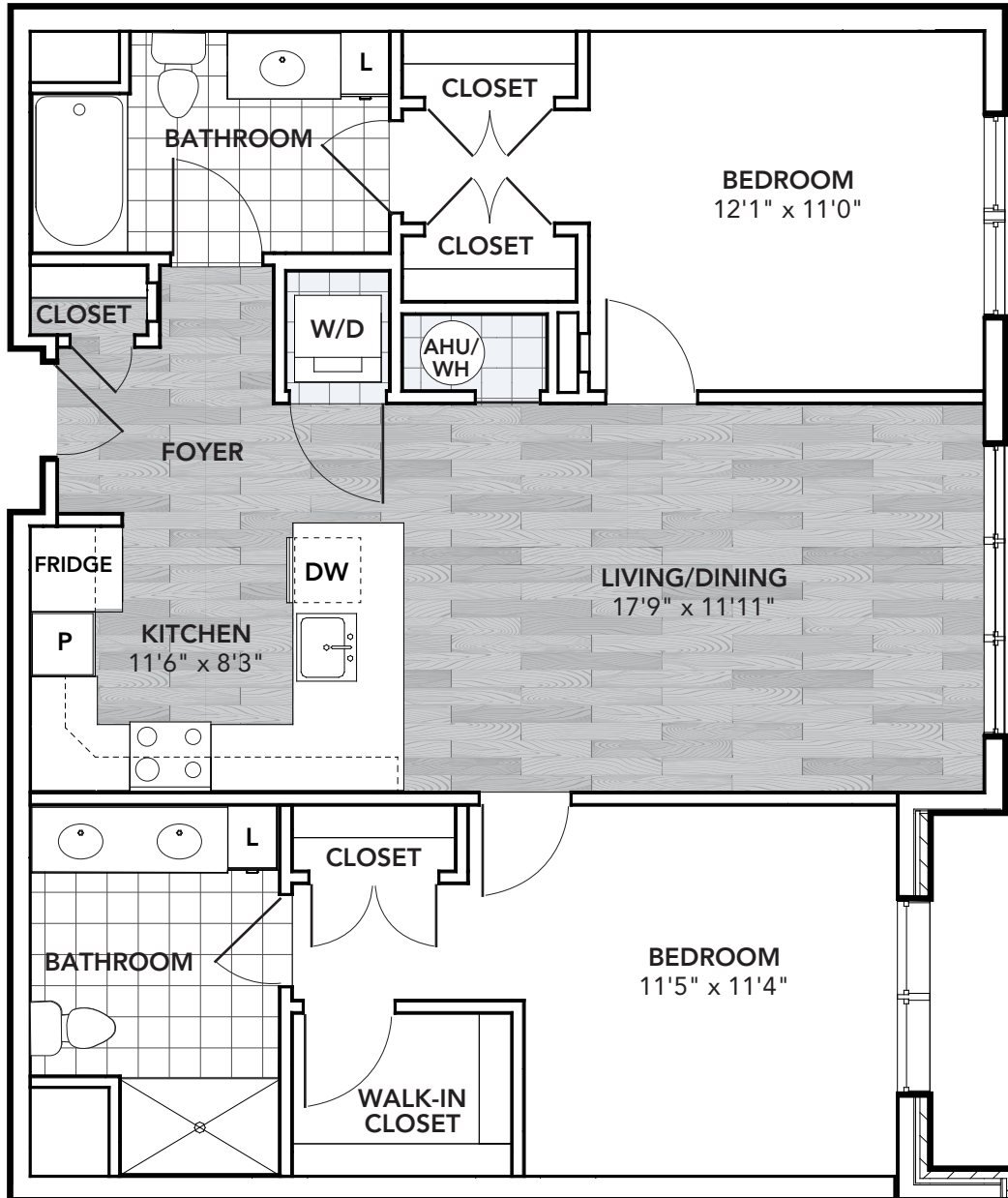
MODEL B3 • 1,071 SQ FT TWO BEDROOM • TWO BATHS
